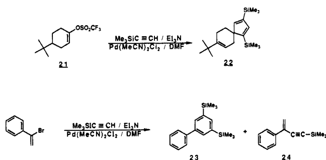
Scheme IV
